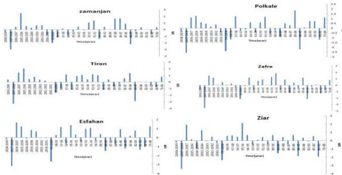
Figure2. SPI diagrams for selected stations in the study area
