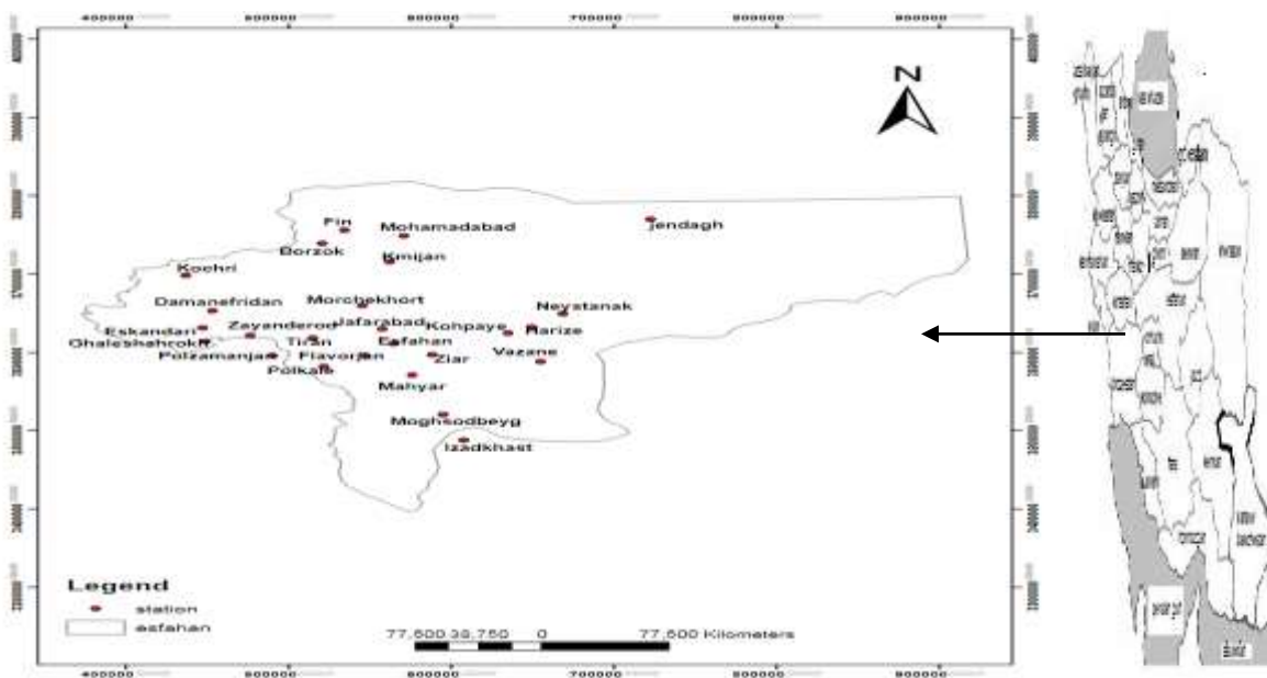
Figure 1. The Esfahan province with identification of the rainfall sites utilized in the study
